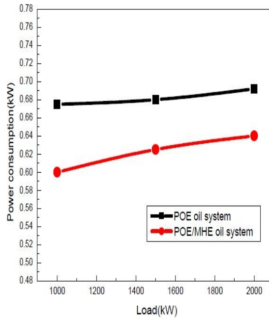
Fig.4 variation of power consumption vs load
