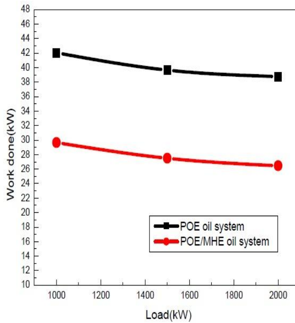
Fig.2 variation of work done vs cooling load
