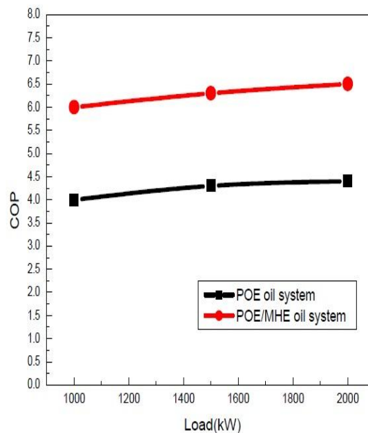
Fig.3 variation of cop vs cooling load
