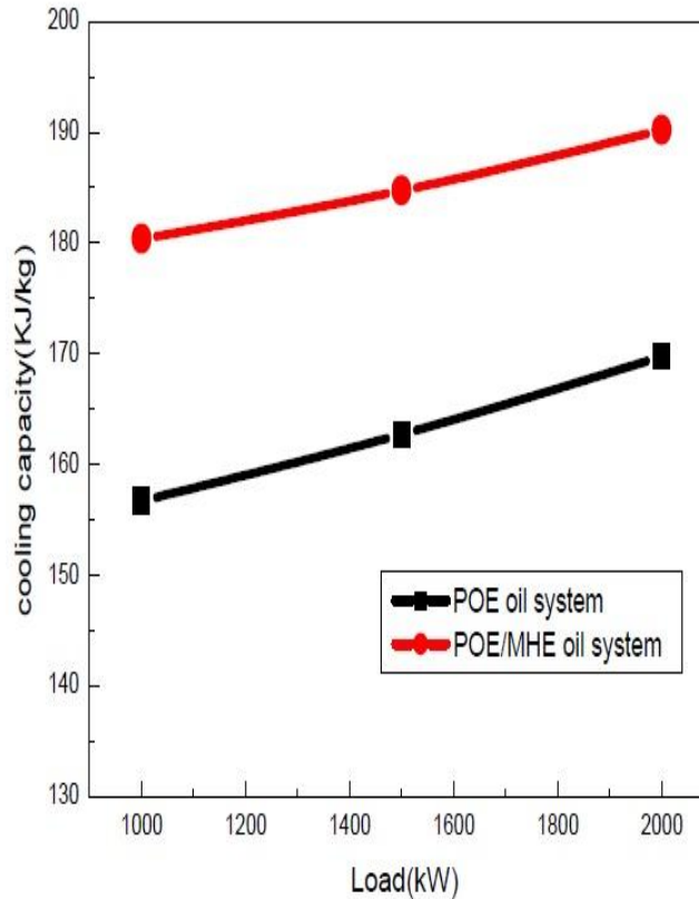
Fig.5 variation of cooling capacity vs cooling load
