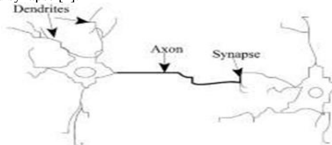
Fig 1: Brain neuron [2]
