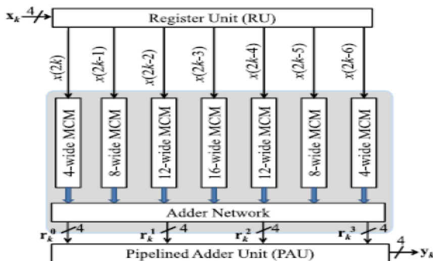
Figure 5: Proposed MCM-based structure for fixed FIR filter of block size L = 4 and filter length N = 16.
