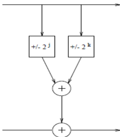
Figure 2: FIR Filter Tap Arithmetic Unit, Coefficients with Two Powers-of-Two
