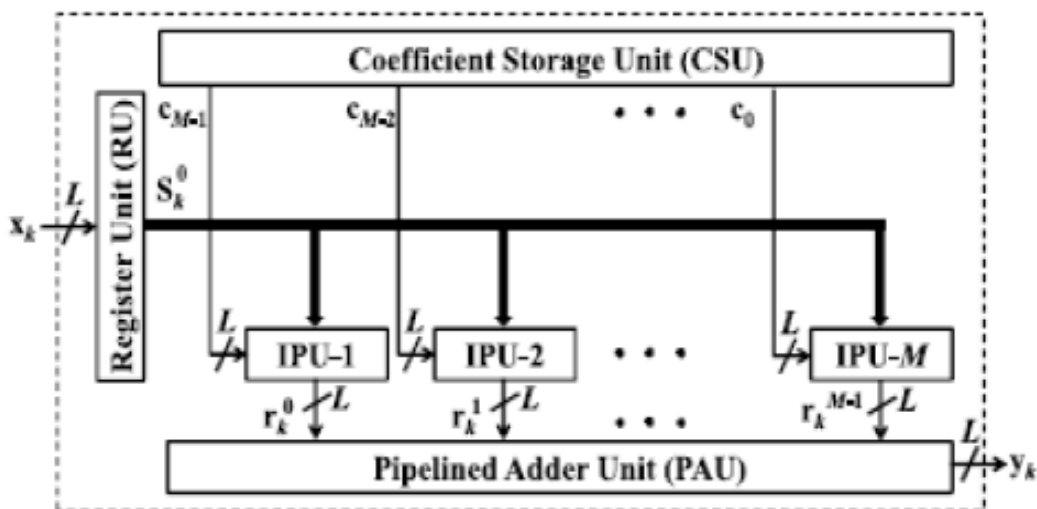
Figure 4: Proposed structure for block FIR filter
