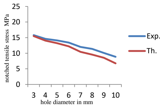
Figure.8. Deviation between theoretical and experimental values
