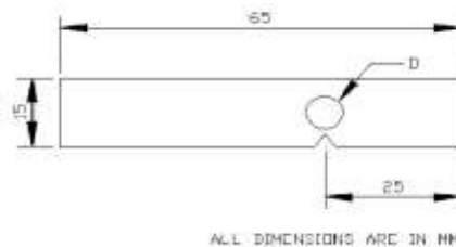
Figure.2.Open hole for impact specimen
