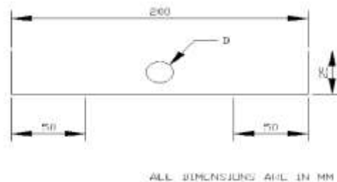
Figure.1.Open hole for tensile specimen
