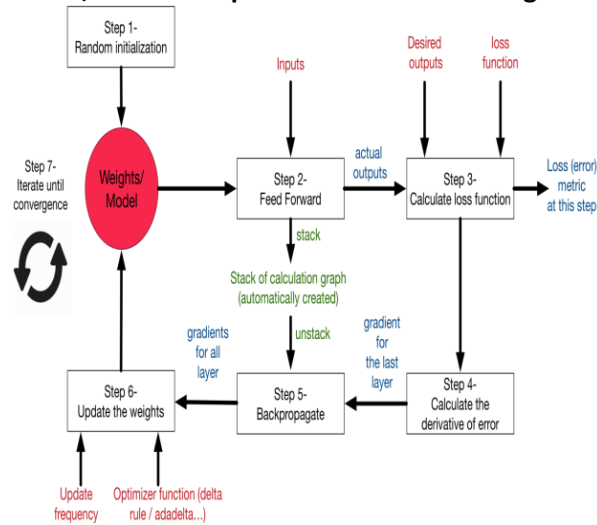
Fig 6: Neural networks step-by-step
