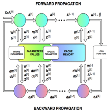
Fig 5: Diagram of Forward and Backward propagation
