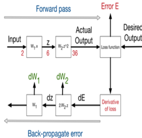
Fig 4: Diagram of Forward and Backward paths
