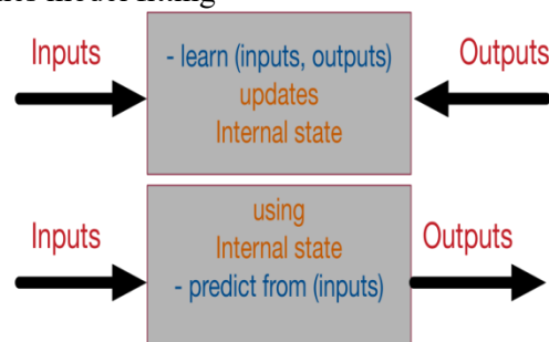
Fig 1: Learning Process
