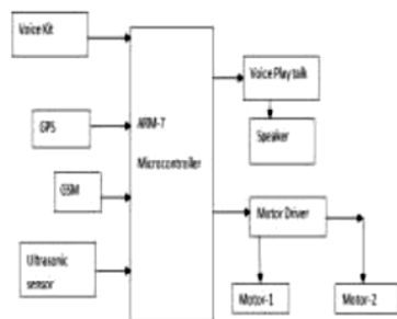
Figure: 1 Block diagram
