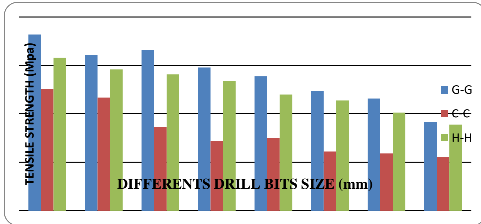
Fig:9 Open Hole Tensile Strength
