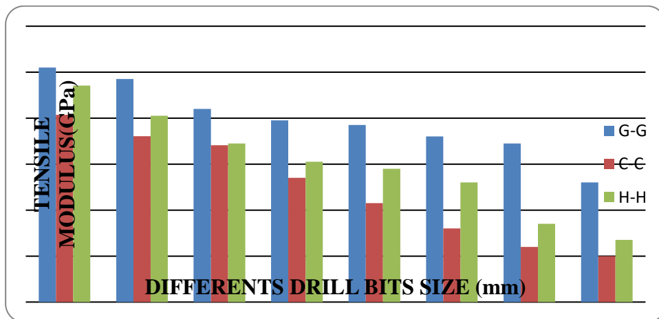
Fig:10 Open Hole Tensile Modulus
